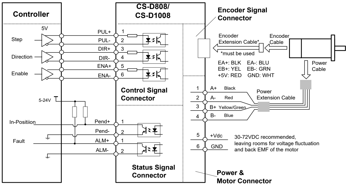
Figure 7: Typical connection
