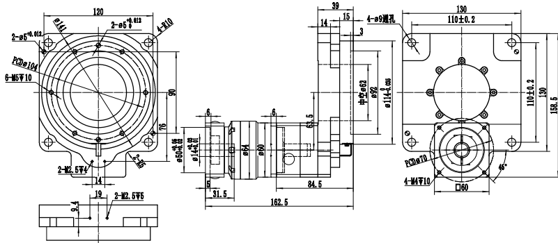
Combined gearbox dimension
