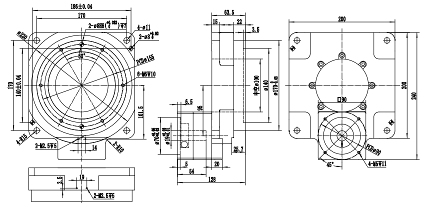
Ratio 10/18 dimension
