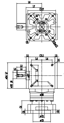
Dimension (double stage, Ratio i=4~20)
