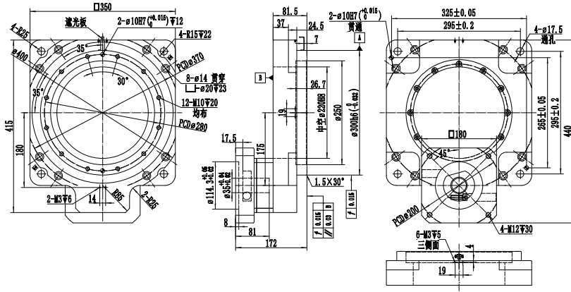
Combined gearbox dimension
