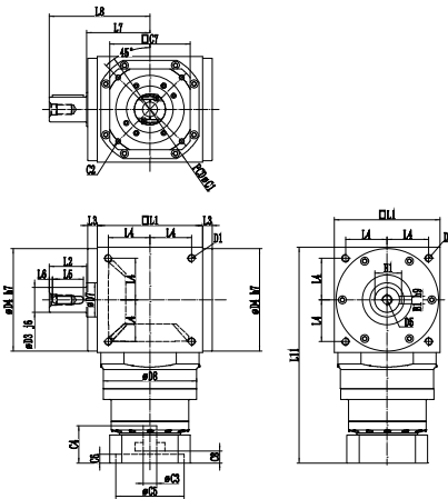
Dimension (3 stage, Ratio i=25~200)
