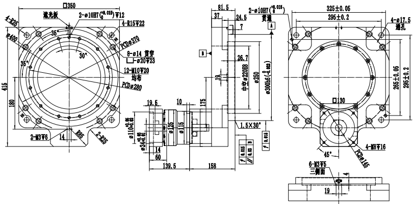
Combined gearbox dimension
